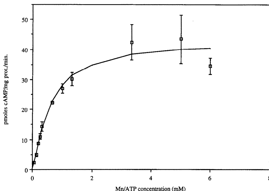
Fig.3. ATP concentration dependence of adenylyl cyclase activity. Activity was measured in the presence of 4.0 mM \text{Mn}(\text{acetate})_2 as a function of ATP added with stoichiometric amounts of \text{Mn}^{2+} . The graph shows the experimental points as the mean \pm SE of 3 independent experiments performed on membranes of strain 975h + . The line shows computer calculated curve that best fit the experimental results and found to show cooperative behaviour (Hill coefficient n_H = 1.68 \pm 0.14 ).
